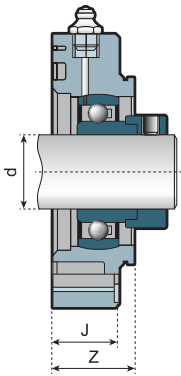
Version with Eccentric Ring
