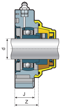
Open Version with Eccentric Ring
