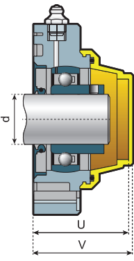
Closed Version with Grub Screws
